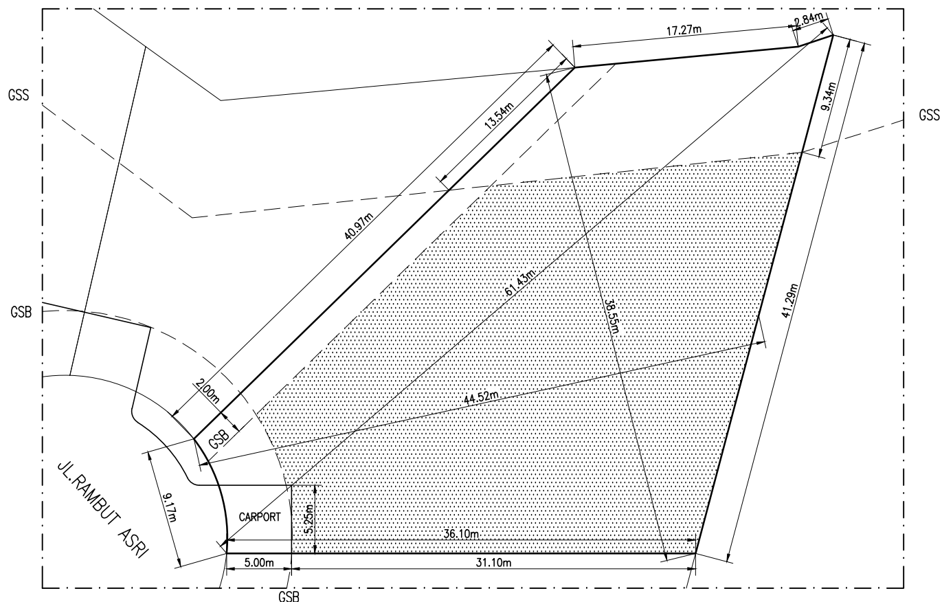
DENAH KAVLING JL.RAMBUT ASRI NO. 5
